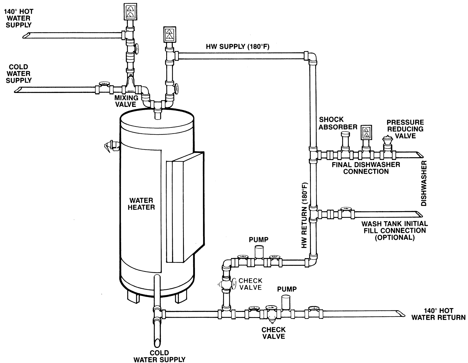
Two Temperature, Single Heater System
