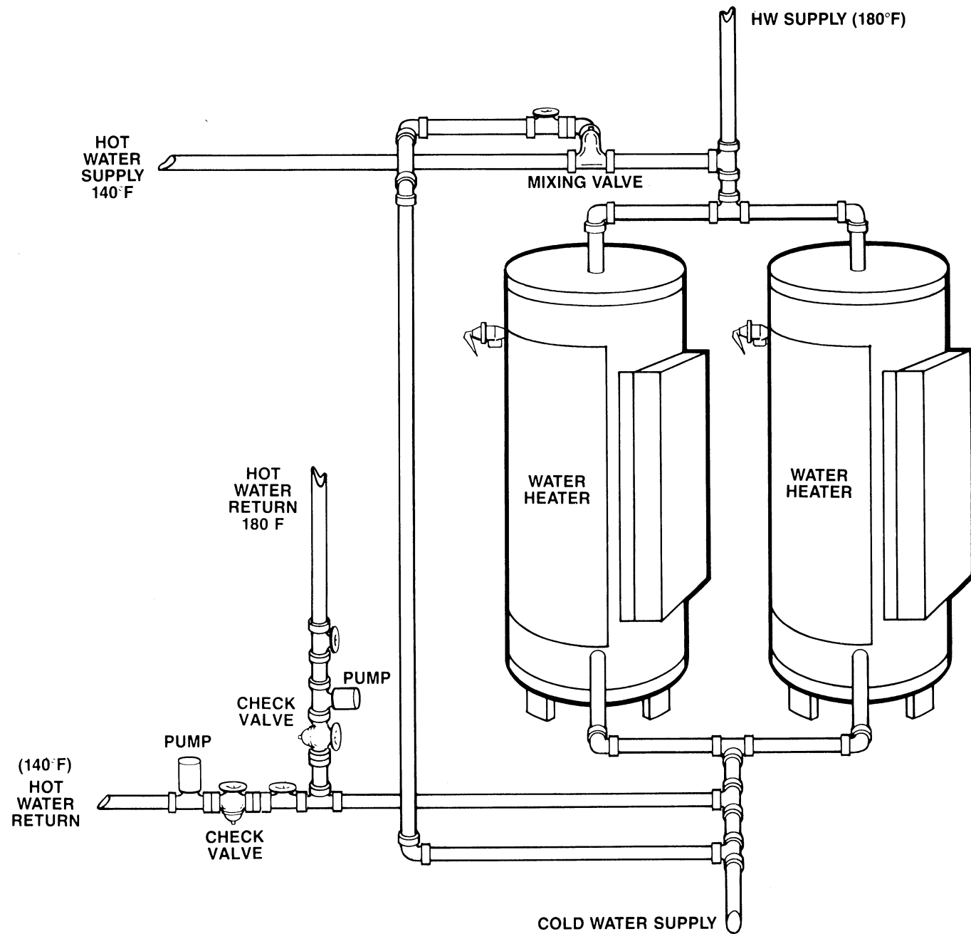
Two Temperature, Dual Heater System (Factory Manifolding)
